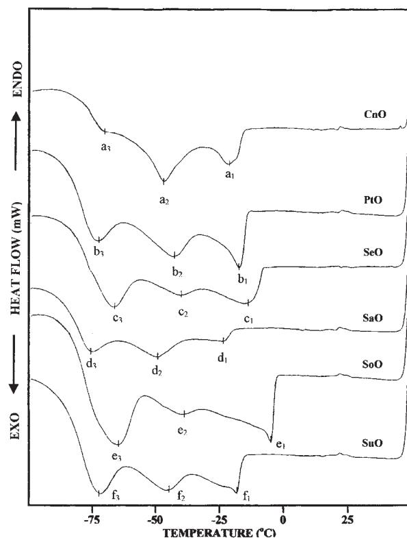
FIG. 3. Differential scanning calorimetry crystallization curves of corn oil (CnO), peanut oil (PtO), sesame oil (SeO), safflower oil (SaO), soybean oil (SoO), and sunflower oil (SuO). Refer to Table 9 for transition temperatures.
