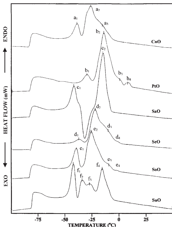
FIG. 7. Differential scanning calorimetry melting curves of CnO, PtO, SaO, SeO, SoO, and SuO. See Figure 3 for abbreviations. Refer to Table 9 for transition temperatures.
